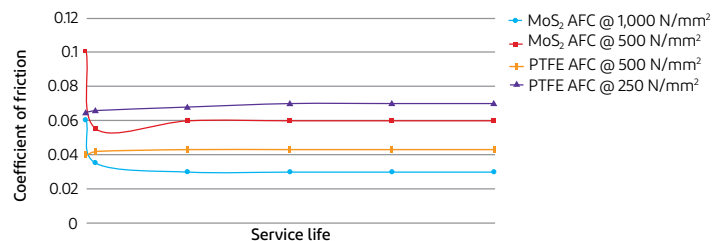
Figure 4. Typical friction values of MoS 2 - and PTFE-based anti-friction coatings under different loads, measured with the LFW1 test machine – ASTM D2714 method.
