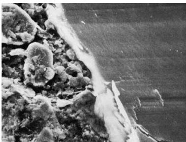
Figure 3. SEM photograph with 1,000x magnification: MoS 2 anti-friction coating before (left) and after (right) load application.
